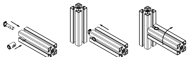
90° CENTRAL CONNECTOR
