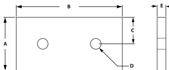
BACKING PLATE-WIDE
