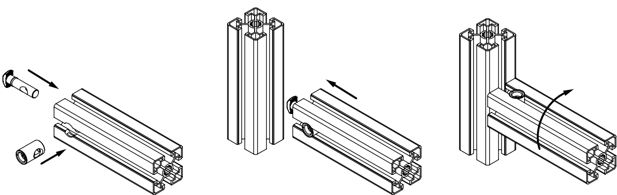
90° CENTRAL CONNECTOR
