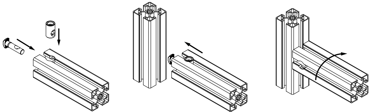
0° CENTRAL CONNECTOR
