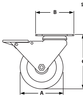
SWIVEL CASTER
