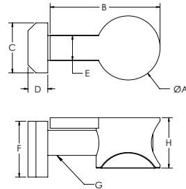
STANDARD TNUT
